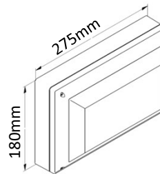
Auge Bulkhead
